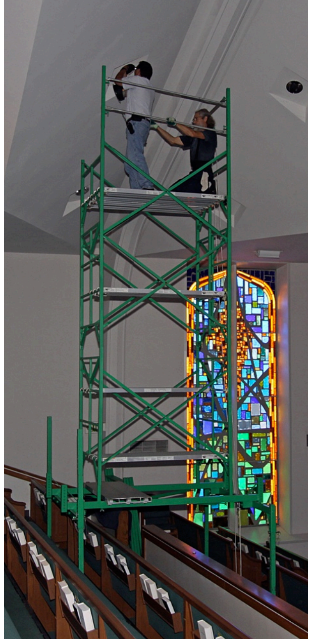
Repairing a light fixture above the stepped balcony in a church. This scaffold was rolled down to the next fixture in about five minutes. The tower was taken down and re-assembled above the next row of pews in about 25 minutes.
